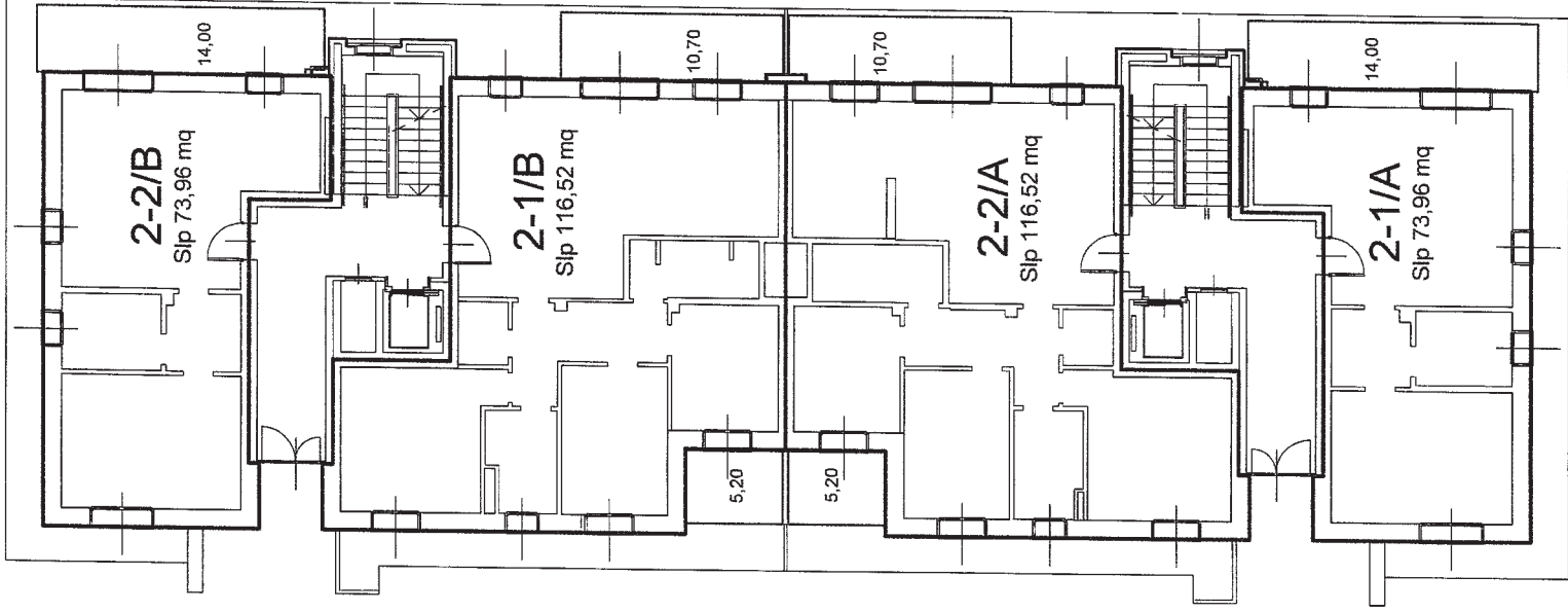
PIANO TERRA
